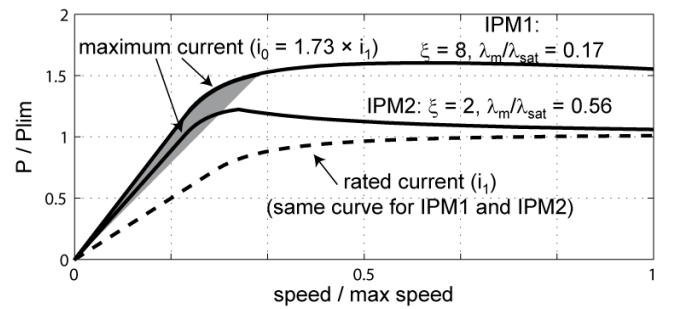
Figure 10. Per-unit power versus speed for two IPM motor drives with different saliency ratio and PM magnet flux, designed for the same continuous torque and power ( T_l , P_l ) according to (10), and with the same rated flux ( \lambda_{sat} ).
