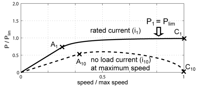
Figure 4. Per-unit power versus speed of the SPM motor at rated current ( i_l ) and no-load current, maximum speed ( i_{10} ).
