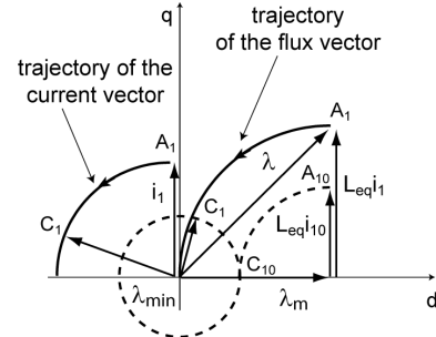
Figure 3. Vector diagram of the SPM motor at rated current ( i_l ) and at the no-load current amplitude needed at maximum speed ( i_{10} ).
