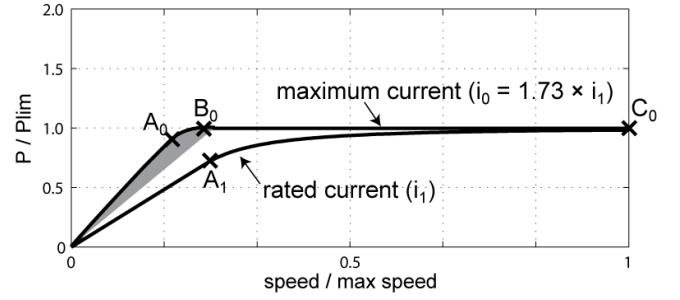
Figure 6. Per-unit power versus speed of the SPM motor at rated current ( i_l ) and 173% overload current ( i_0 ).
