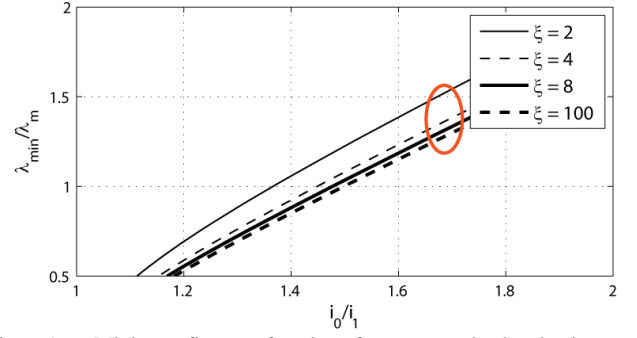
Figure 9. Minimum flux as a function of current overload and anisotropy ratio.
