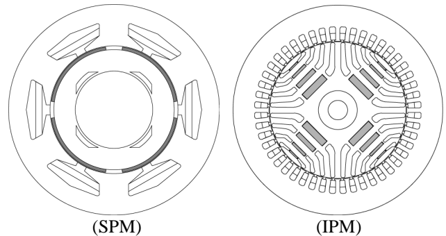
Figure 1. Example motors, having the same continuous torque, power and current ( P_t , T_t , i_t ). The two motors have the same stator diameter and stack length.
