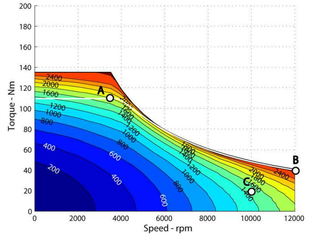
Figure 13. Total loss map of the SPM motor. The white line refer to the continuous current i_1 = 208 A (pk), the outside limit of the map refer to the overload current i_0 = 360 A (pk). PMs at 100° C. Copper at 130° C.
