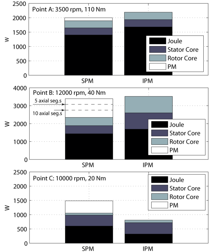
Figure 17. Detail of motor losses in the three working points A, B, C circled in Figs. 13-16.
