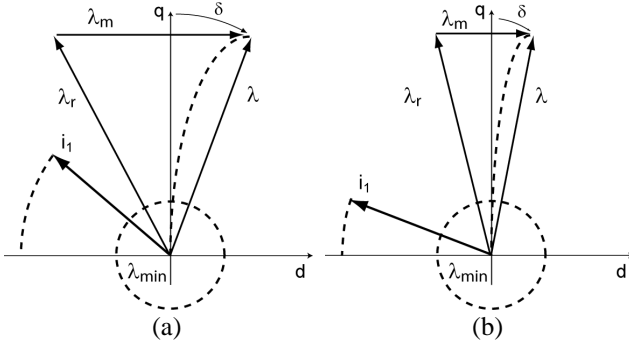
Figure 7. Vector diagrams of two IPM motors at rated current ( i_l ), in the respective MTPA conditions. The dashed curves are the trajectories of the flux and current vectors in flux weakening. a) motor with low anisotropy. b) motor with high anisotropy.
