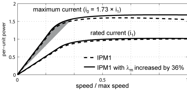
Figure 11. Effect of increased PM flux on overload capability: per-unit power vs speed curves for IPM1 (same as Fig. 8) and IPM1 with PM flux increased by 36% according to (13).
