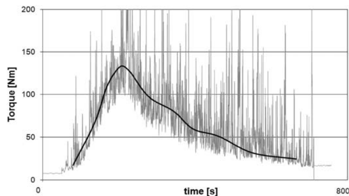
Fig. 5. Obtained diagrams of the recorded torque for the conditioned Turin soil
