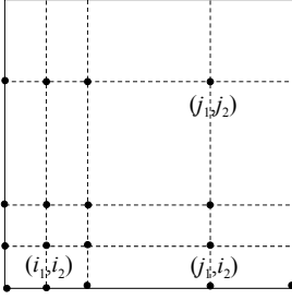
Fig. 1 A representation of the bivariate rectangular lattice \mathcal{X}_2 = \{1, 2, \dots, l\}^2
