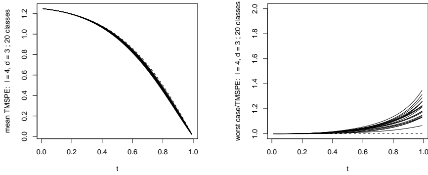
Fig. 3 Performance of LHDs for l = 4 and d = 3
