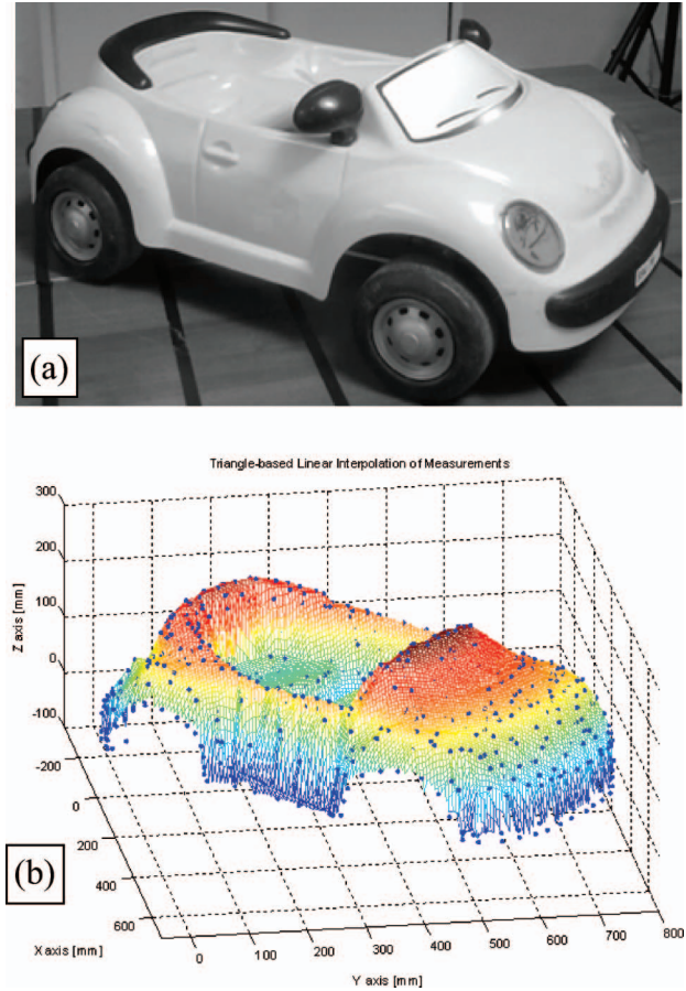
Figure 9. (a) Toy car model. (b) Measured points and reconstructed shape.
