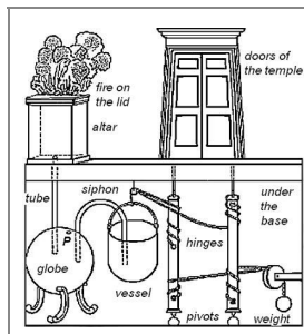
Figure 3. When the fire on the altar has grown hot, the pressure in the globe increases, driving out some liquid contained there through the siphon into a suspended vessel. The vessel, descending under the weight, will tighten the chains and open the doors. When the fire is extinguished, the pressure decreases, the water flows back into the globe through the bent siphon from the suspended vessel. The weight suspended will preponderate and shut the doors.
