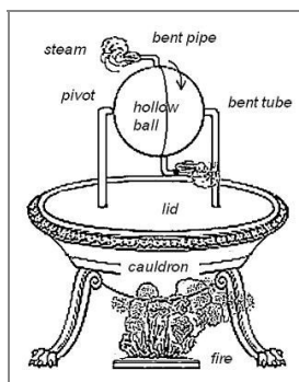
Figure 1 Aeolipile or the Hero's Machine. Heating the water in the cauldron with a fire, the steam enters the hollow ball through the bent tube and passes out through the two bent pipes, causing the ball to revolve.
