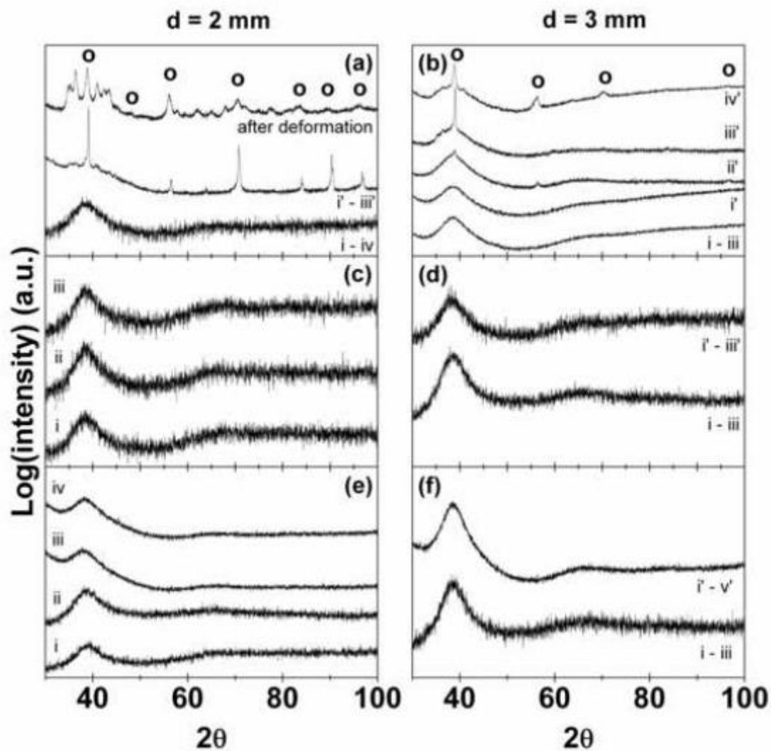
Fig. 1. Selected XRD patterns of different rods from the as cast rods. (a) and (b): \text{Cu}_{48}\text{Zr}_{48}\text{Al}_4 with 2 and 3 mm diameter, respectively; (c) and (d): \text{Cu}_{47.5}\text{Zr}_{47.5}\text{Al}_5 with 2 and 3 mm diameter, respectively; (e) and (f): \text{Cu}_{46.5}\text{Zr}_{46.5}\text{Al}_7 with 2 and 3 mm diameter, respectively.
