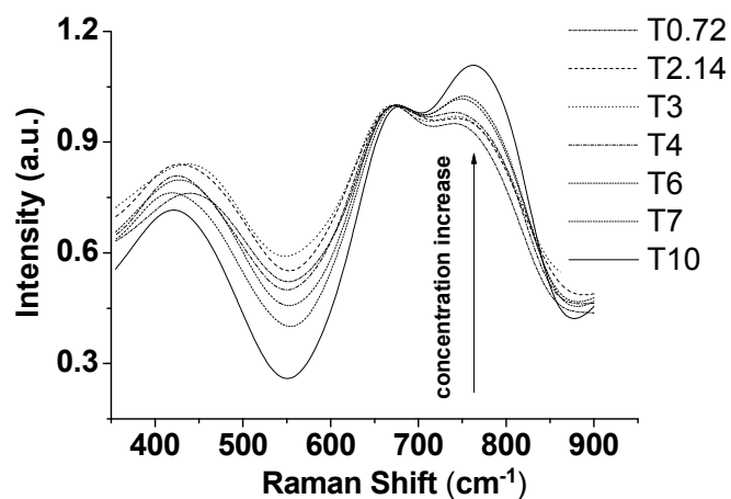
Figure 1. Raman spectra normalized to the peak at 650\text{ cm}^{-1} . Excitation wavelength was 1064 nm [From Ref.9].
