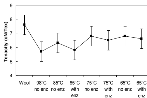
Figure 6. Tenacity measurements on wool yarn dyed in different conditions.
