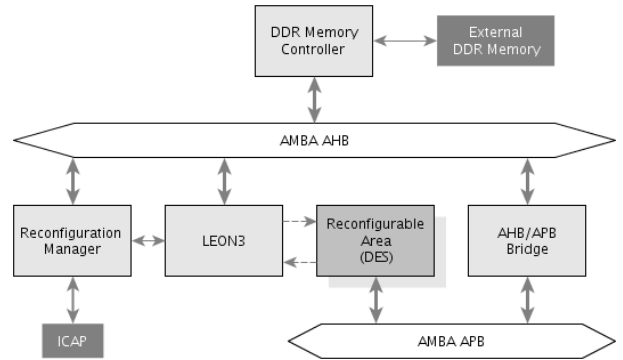
Figure 3. Conceptual block diagram of the proposed architecture
