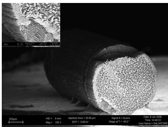
Fig. 2: Cylindrical CNTs bunch laid down on a silicon surface.
