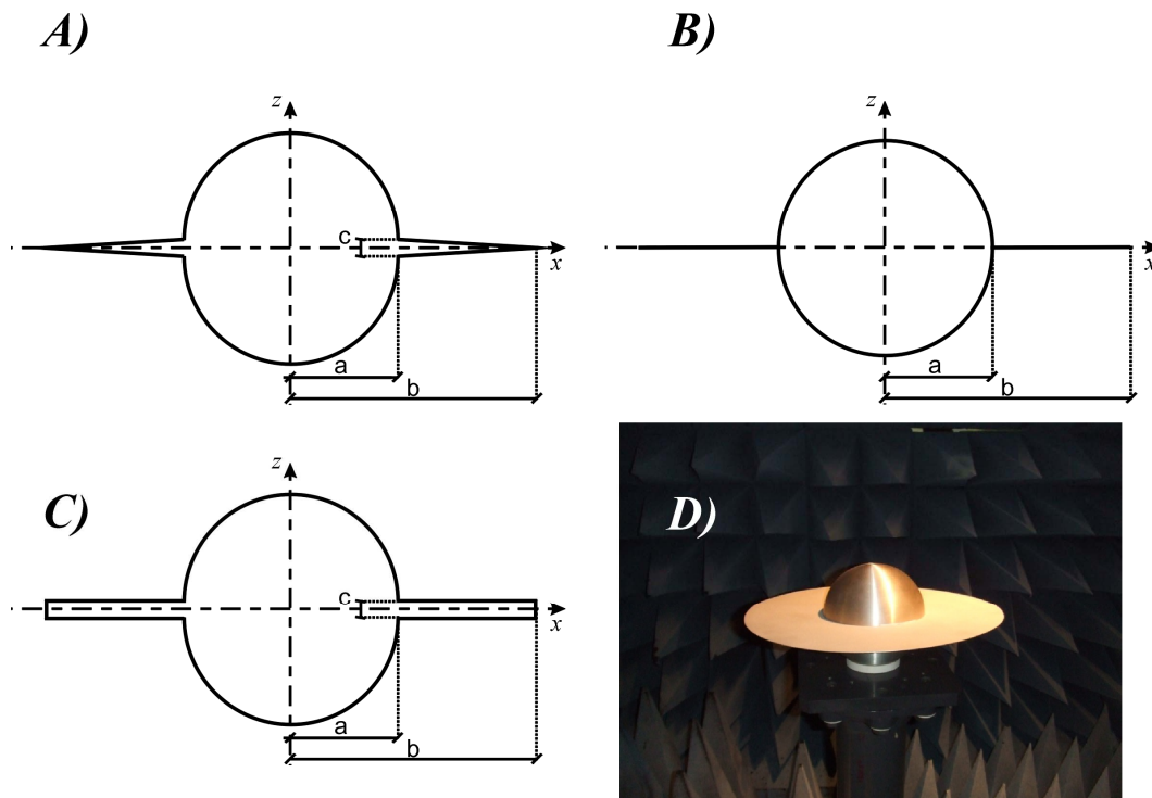
Fig. 1: A, B, C) Cross sectional view of the models for a metal sphere with disks of decreasing thickness, zero thickness, and finite thickness, respectively; D) Aluminum manufactured sphere with disk of radius a=76\text{mm} , radius b=190\text{mm} , thickness c=1\text{mm} .
