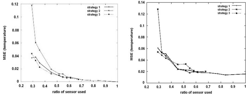
(a) T_{model} 8524-9160 epochs
