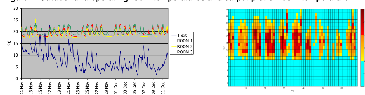
Figure 7. Outdoor and operating room temperatures and carpet plot of room temperature.
