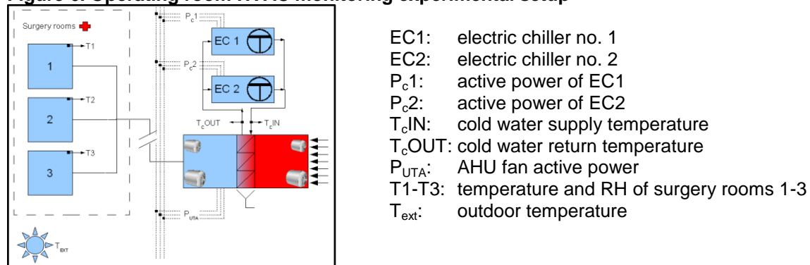
Figure 6. Operating room HVAC monitoring experimental setup
