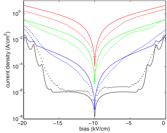
FIG. 5. (Color online) Comparison between computed IV curves (lines) and experimental data (dots) at temperatures of 10 (black), 40 (blue), 50 (green), and 60 K (red).
