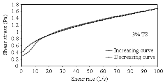
Fig. 2a: Double repeated ramp test results (3% TS sludge without polyelectrolyte)
