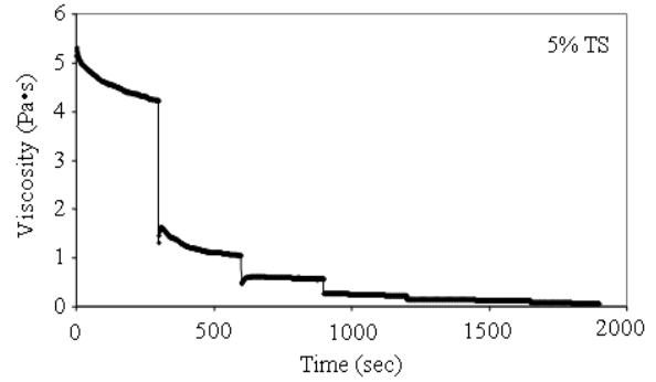
Fig. 7b: Step-test results (5% TS sludge without polyelectrolyte)
