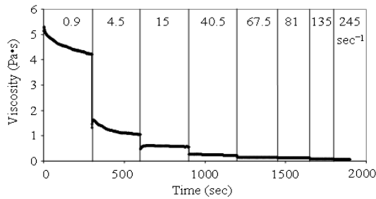
Fig. 6: Example of step-test results
