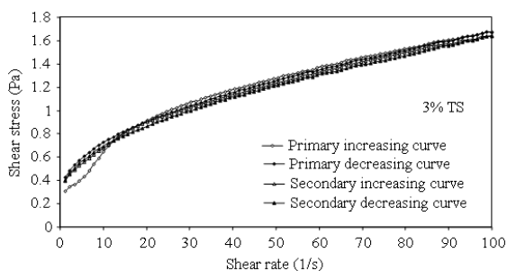
Fig. 4a: Double repeated ramp test results (3% TS sludge without polyelectrolyte; primary and secondary test)
