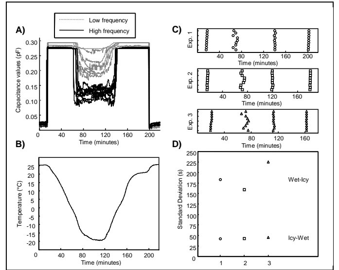
Figure 4. Statistical analysis of laboratory data. (A) Values of capacitance (raw data) obtained for each sensor during the first experiment. (B) Internal temperature of the climatic chamber during the first experiment. (C) Time instants of state transitions estimated for each sensor during 3 experiments. (D) Standard deviations of time instants of state transitions wet-icy and icy-wet estimated for each sensor during 3 different experiments.
