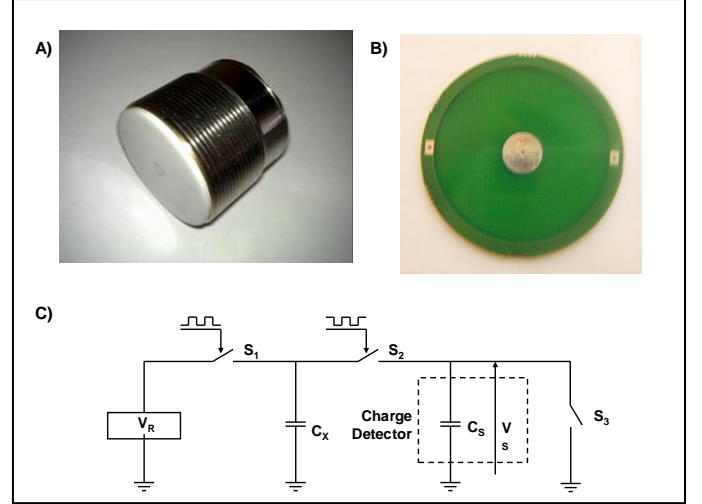
Figure 2. The ice sensor. (A) Picture of the ice sensor. (B) Picture of the concentric conductive electrodes. (C) Schematic layout of the capacitive measurement circuit.
