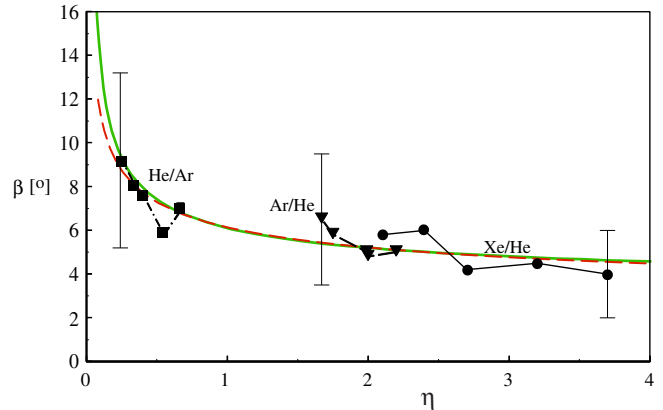
FIG. 12: Spreading angles of intermediate jets vs density ratio (the axial Mach number downstream from the Mach disk is about 0.45 for all the jets). The green line is a fit according to Papamoschou and Roshko (1988) (the red dashed line is the best scaling law fit, see formula (13)).
