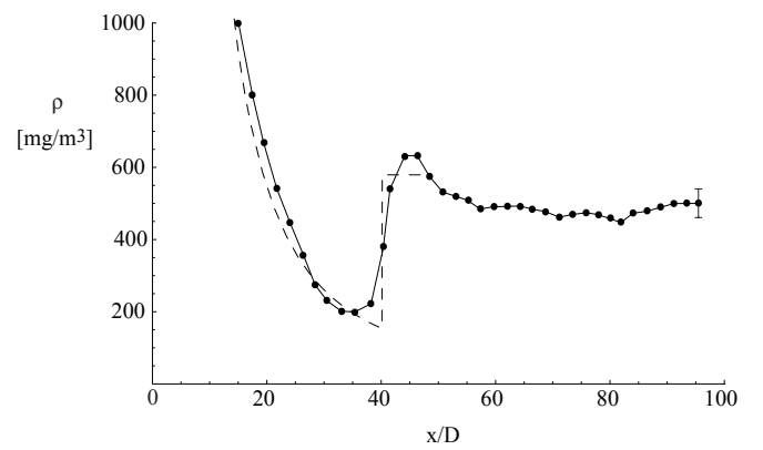
FIG. 5: Axial density for the Xenon jet visualized in fig. 4. A sample error bar is shown on the right. The zone on the left cannot be analyzed because of the high density values (saturated output). The dashed line shows, as a reference, an equivalent isentropic expansion followed by a normal shock.
