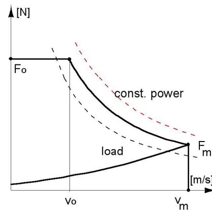
Fig. 2 – Required constant-power speed range.
