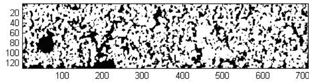
Thresholded original BSE/SEM Image - Porous LSM current collector
