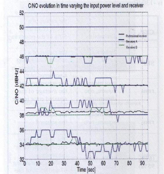
Fig.5: C/N_0 estimation varying with time and with the input power level evaluated for different GPS receivers
