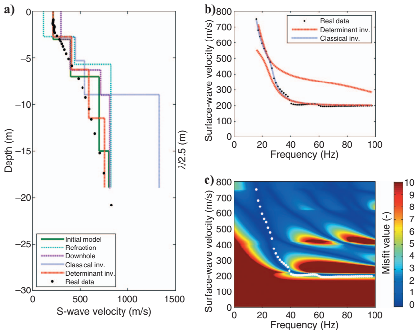
Figure 13. Inversion results for site B, Castelnuovo, Garfagnana, Italy. (a) S-wave velocity profiles compared with the first branch of the real data ( \lambda/2.5 - V domain), a downhole test result, and a refraction result. (b) Dispersion curves. (c) Real dispersion curve compared with the misfit surface of the determinant approach.
