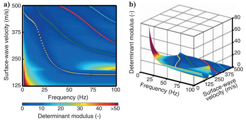
Figure 1. Absolute value of the Haskell-Thomson determinant for a given model (three layers over a half-space, water layer on top of the model). Colored dots represent the modal curves that correspond to the zeros of the determinant. The minima of the surface correspond to the dispersion curves of the model: (a) 2D view; (b) 3D view.
