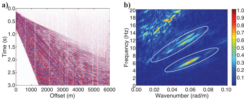
Figure 10. Representation of (a) the recorded seismogram and (b) the corresponding f-k spectrum of the seismogram for site A (marine data). The white circles represent the regions where the dispersion curve is picked.
