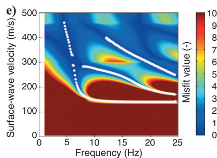
Figure 5. Inversion results for synthetic case 1. (a) The S-wave velocity profiles for the inversion of the slowest branch of the dispersion curve compared with the first branch of the synthetic data ( \lambda/2.5 - V domain). (b) Dispersion curves for inverting the slowest branch of the dispersion curve. (c) S-wave velocity profiles for the inversion of all curve branches compared with the first branch of the synthetic data (classical inversion is coincident with the true model). (d) Dispersion curves for the inversion of all curve branches. (e) Synthetic dispersion-curve compared with the misfit function of the determinant inversion.
