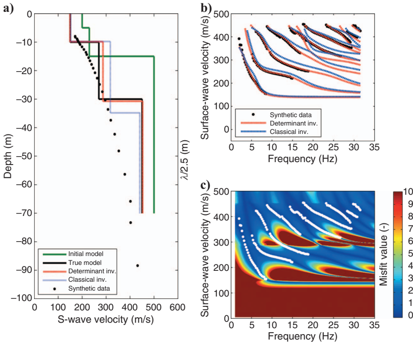
Figure 9. Inversion results for synthetic case 2. (a) S-wave velocity profiles compared with the first branch of the synthetic data ( \lambda/2.5-V domain). (b) Apparent dispersion curves compared with the calculated dispersion curves for the final models. (c) Apparent dispersion curve compared with the misfit function of the determinant approach.
