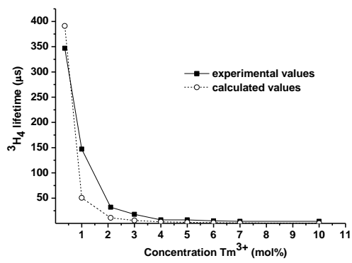
Fig. 8. Calculated and measured lifetime values of the ^3H_4 level. Deviation from experimental values is smaller for higher dopant concentrations.
