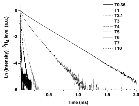
Fig. 4. Lifetime decay curves of {}^3\text{H}_4 level. Exponential decay is only in the case of sample T0.36
