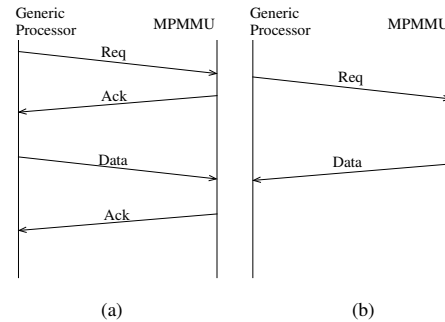
Fig. 4. Write (a) and Read (b) protocol between a processor and the MPMMU
