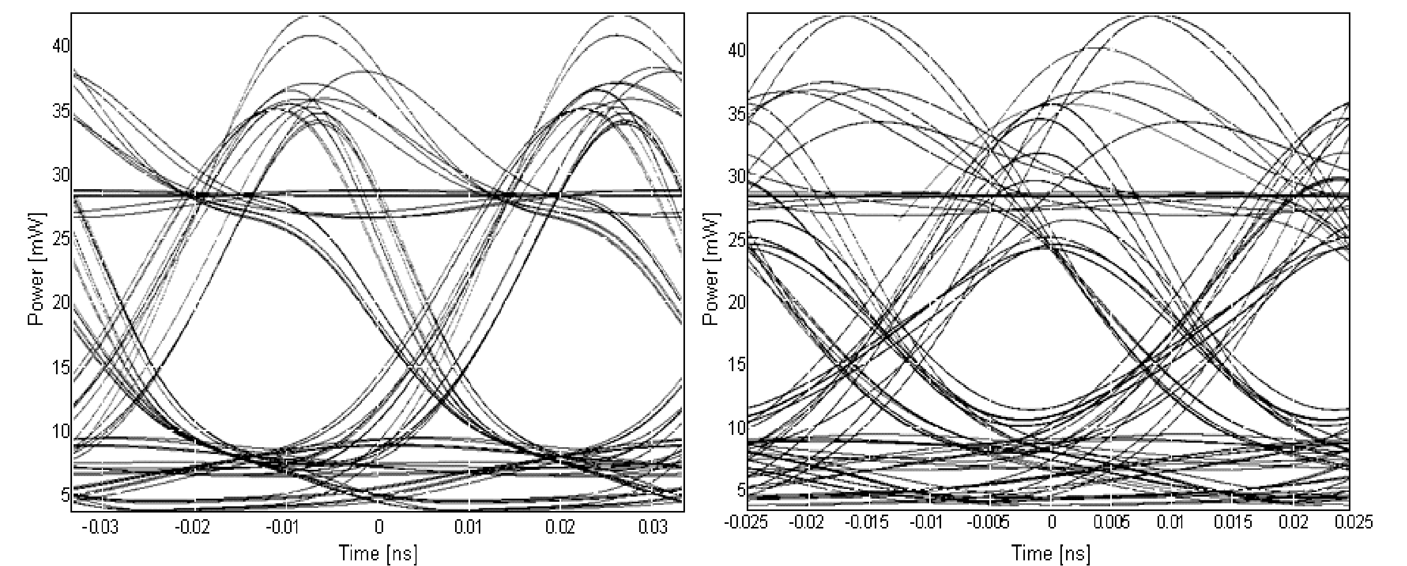
Fig. 5. Eye diagrams calculated at the optimal EMB condition ( n_{\text{eff,grat}}=3.246 ) with a NRZ PRBS signal with 33 \text{ Gbit/s} (a) and a 40 \text{ Gbit/s} (b) bit rate.
