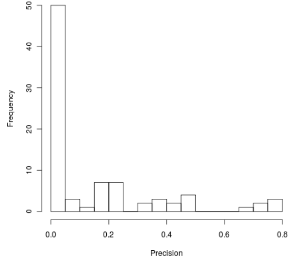
Figure 1. Hystogram of precisions
