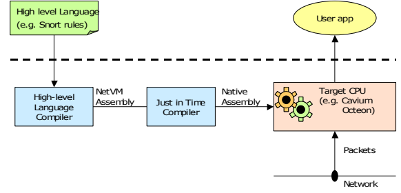
Figure 2. The code generation process in NetVM.
