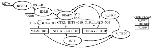
Fig. 8. Simplified flow diagram of the control block.
