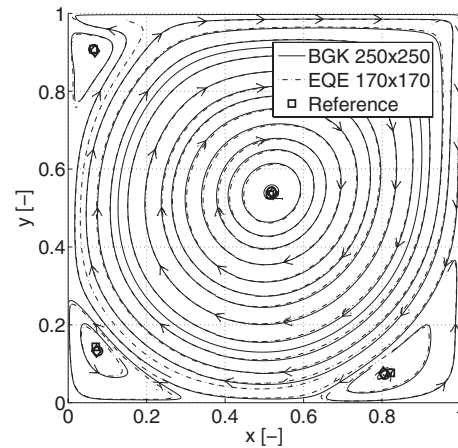
FIG. 5. Streamlines for the lid driven cavity flow with Re = 5000 , \nu=0.0002 ( \xi=0.002 for the EQE model only). The reference locations x_q^r for the four main vortexes are reported [25–28] (square markers). Moreover the computed locations x_q based on the postprocessing are reported too for both BGK (circle markers) and EQE model (diamond markers).
