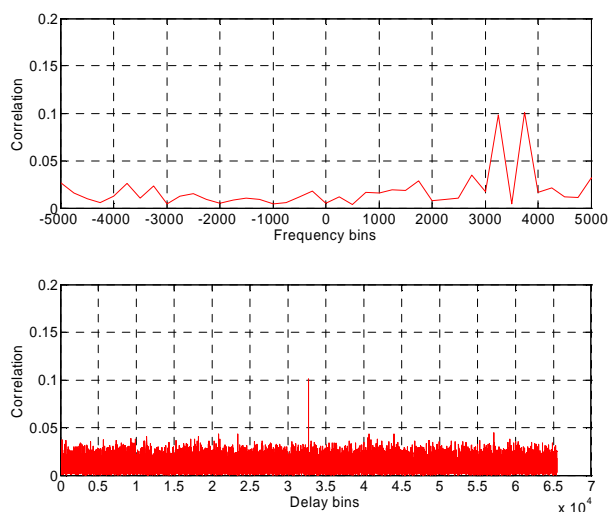
Figure 4: Curves extracted from the CAF envelope in case of with bit sign transition.
