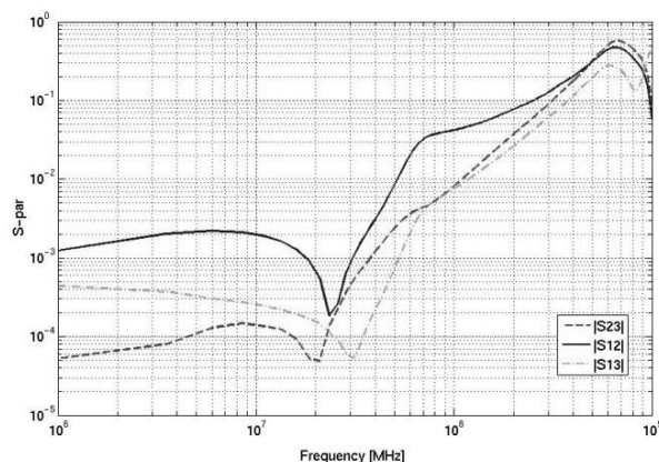
Fig. 4 Transmission scattering parameter between the power supply of core logic (port #1) and a power the drain of two different power transistors (ports #2 and #3) integrated in the same chip.
