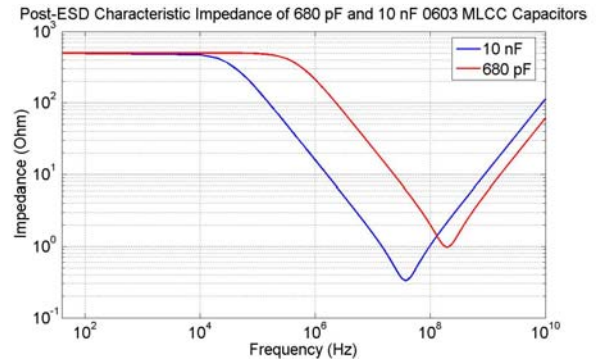
Fig. 10. Simulated Post-ESD Impedance Characteristics, R3 = 500 Ω
