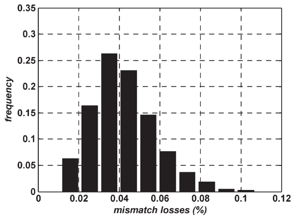
Fig. 17. Mismatch losses (P-220) for 1000 strings.
