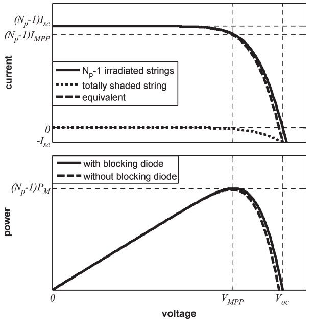
Fig. 12. Effect of blocking diodes.
