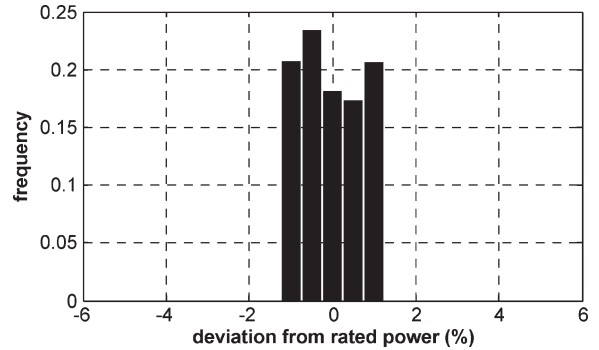
Fig. 14. Power dispersion of P-220 modules.
