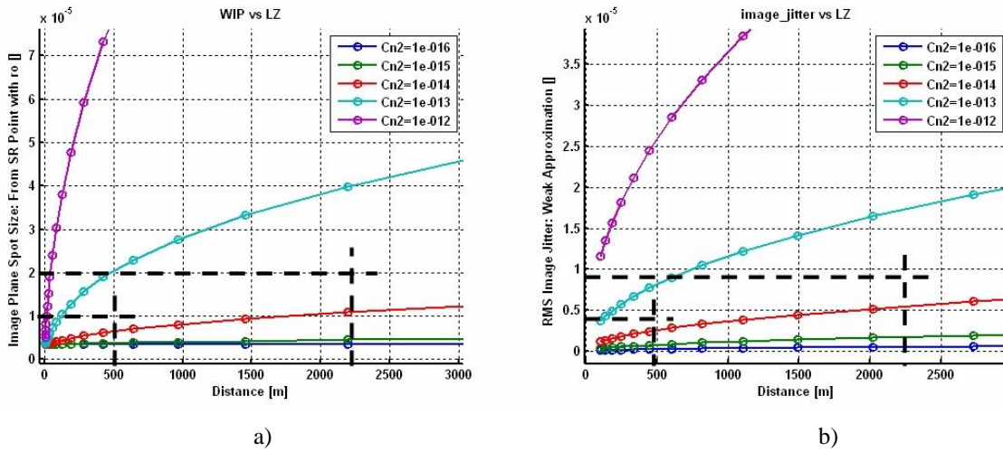
Fig. 4. a) Spot size radius at the image plane and b) rms jitter due to angle of arrival fluctuations.
