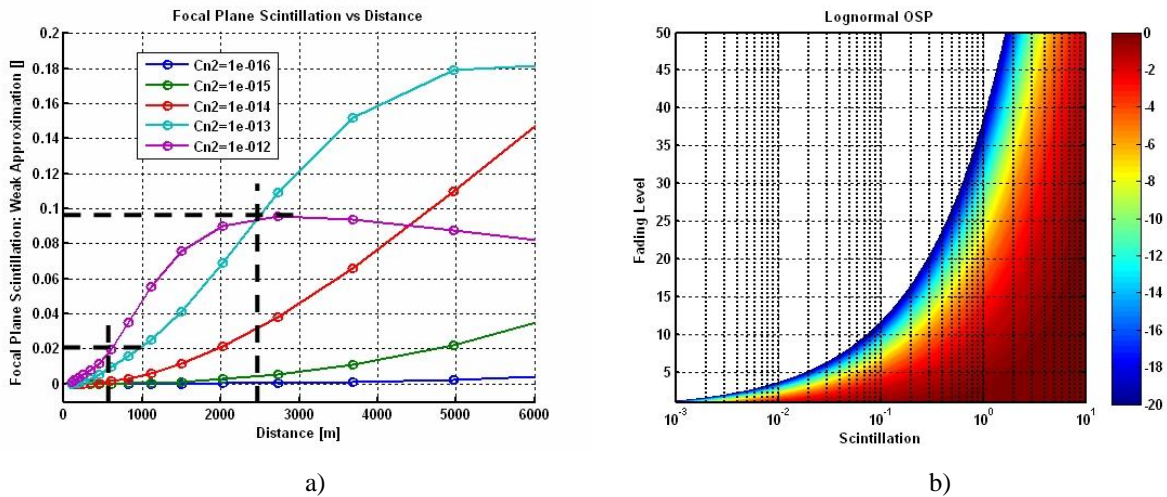
Fig. 3. a) Scintillation at the image plane and b) log normal fade level
