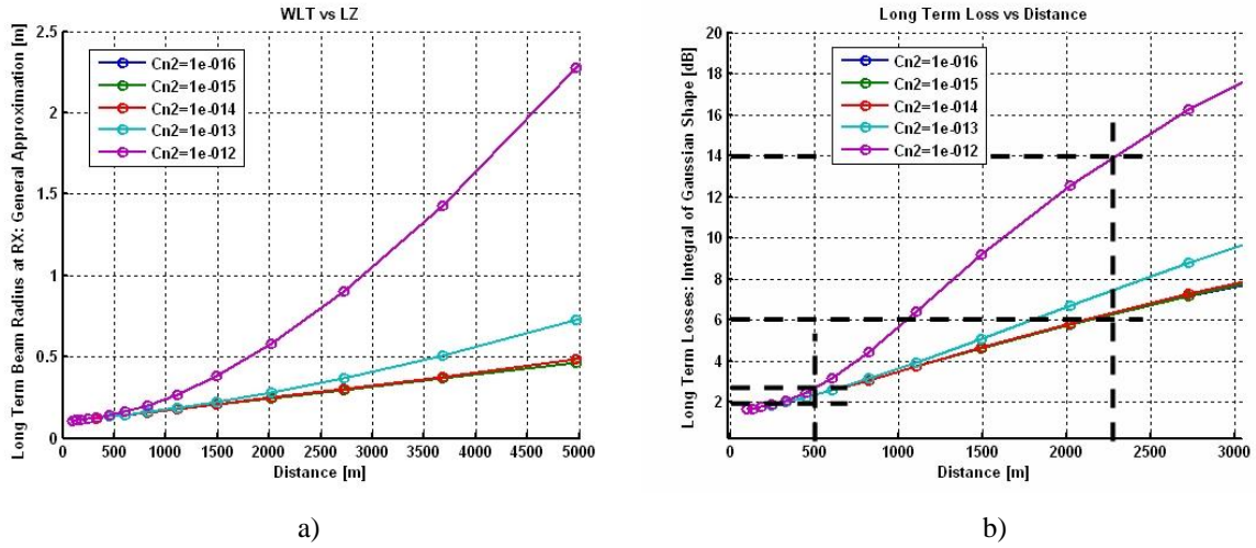
Fig. 2. a) Long term beam spread that takes into account beam wander and short-beam spread and b) long term losses due to the finite telescope aperture size.
