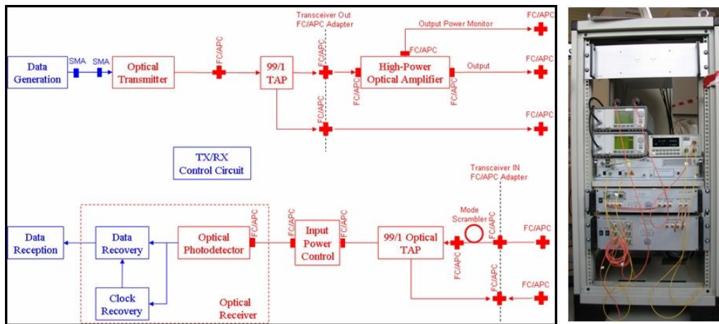
Fig. 6. Transceiver design.
