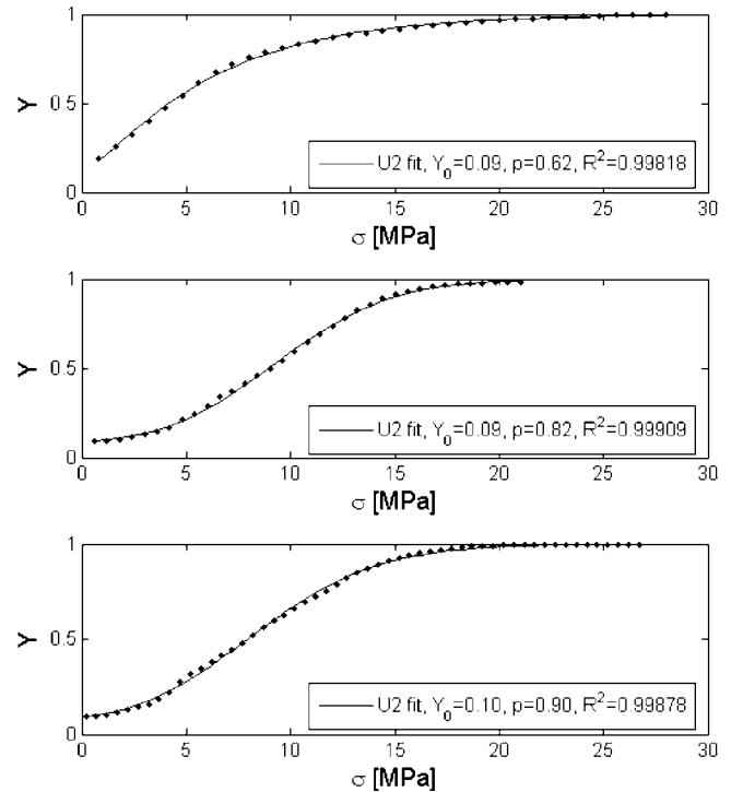
FIG. 4. Simulated damage factor Y (dots) vs applied stress for different values of the Weibull modulus: m = 0.7, 1.7 , and 2.5 starting from the top, respectively. The data are fitted with Eq. (6). The excellent values of R^2 confirm that the analyzed phenomenology belongs to the PUN U2 class.
