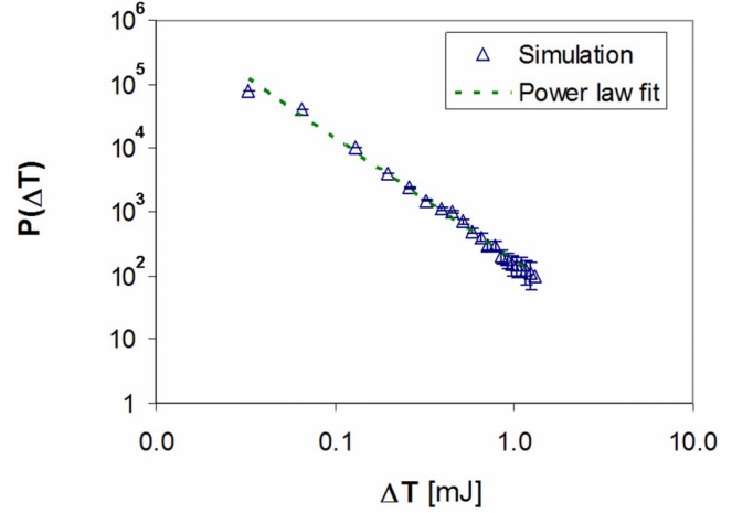
FIG. 2. (Color online) Distribution P(T) of the simulated released AE energy T during damage progression in a virtual specimen. Simulation data include error bars.
