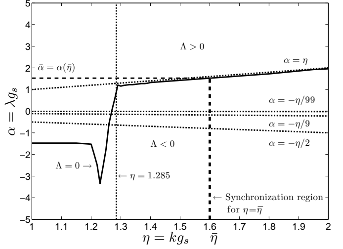
Fig. 1. Sign of the modified MSF with bounds on the second eigenvalue of \mathbf{G} (dotted lines) and synchronization region (dashed bold line) corresponding to \eta = \bar{\eta} .
