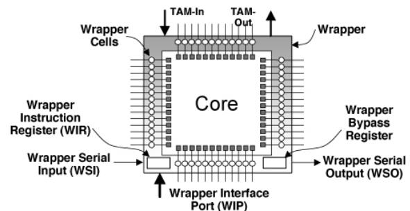
Fig. 1. IEEE std. 1500 Core Test Wrapper Architecture
