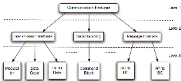
Figure 2. MIL - STD 1553 Features
