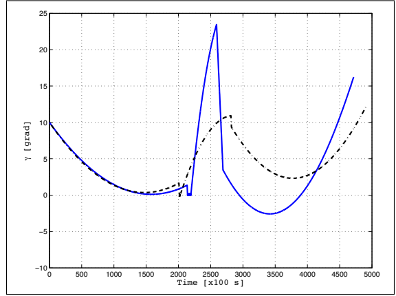
Figure 12: Climb Turn Trajectory: Climb Angle.
