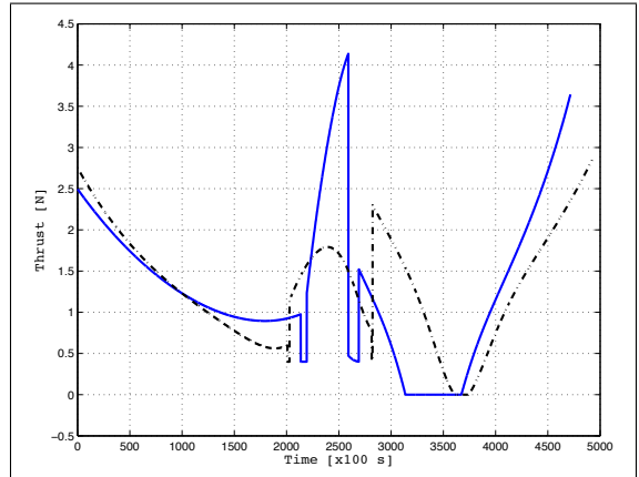
Figure 13: Climb Turn Trajectory: Thrust.
