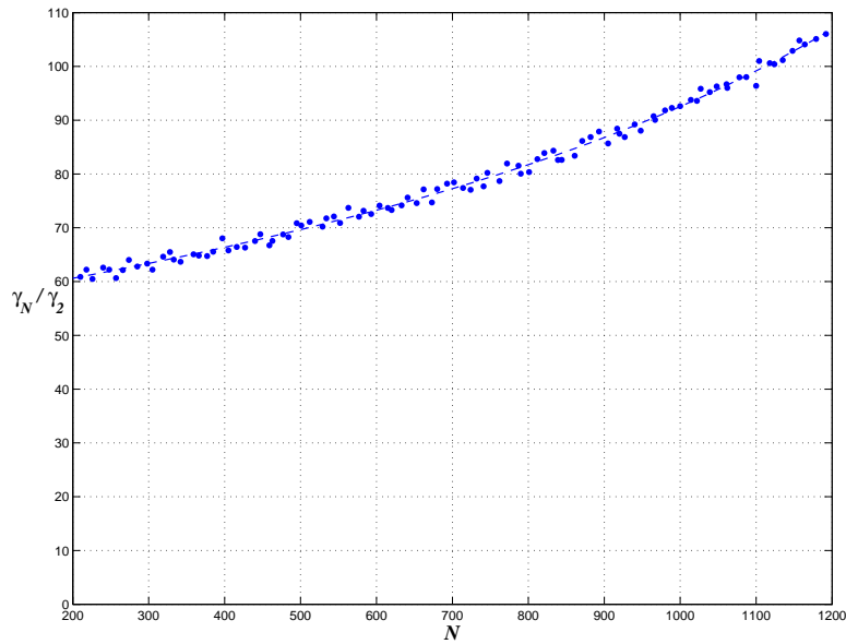
Fig. 3. \gamma_N/\gamma_2 versus N for the model M(N, \beta, d, m) with \beta = 3 , d = 7 , and m = 30 .
