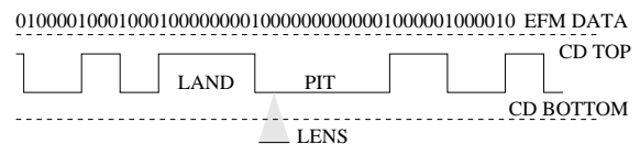
Figure 1. CD pits and lands stored data.
