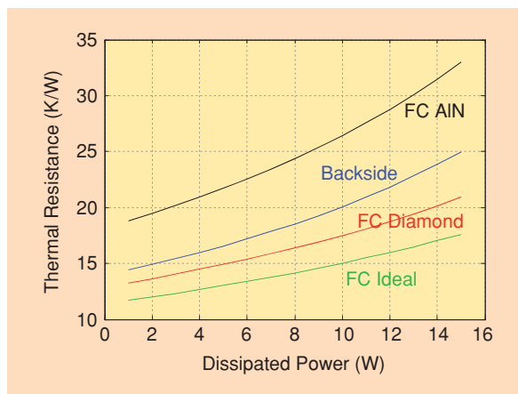
Figure 3. Thermal resistance of an AlGaN/GaN device as a function of the dissipated power and for different mountings setups [25].
