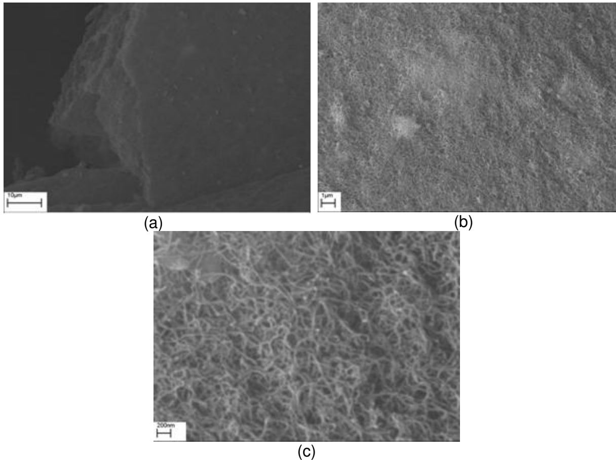
Fig. 5. SEM micrograph of PE10 cone residues a) 10 µm size mark b) 1 µm size mark c) 200 nm size mark
