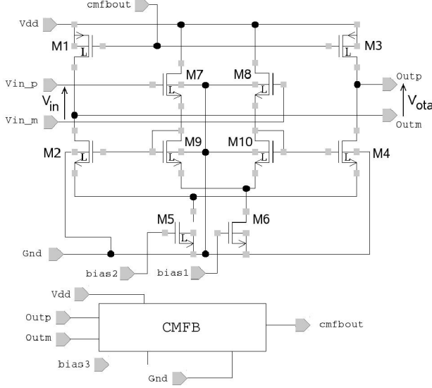
Fig. 4. Schematic of the Transconductance Amplifier
