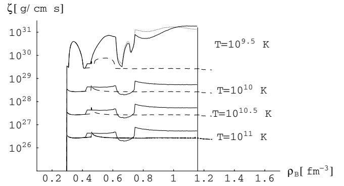
FIG. 3. Bulk viscosity in the first scenario as a function of baryon density for various temperatures. Solid lines refer to MP viscosity, while dashed lines correspond to pure hyperonic matter (vanishing hyperon gap in the upper panel and finite hyperon gap in the lower panel). The dotted lines corresponds to the case in which a large hadron-quark surface tension ( 10 \text{ MeV/fm}^2 < \sigma < 30 \text{ MeV/fm}^2 ) is taken into account and they are computed for T = 10^{9.5} \text{ K} (see text).
