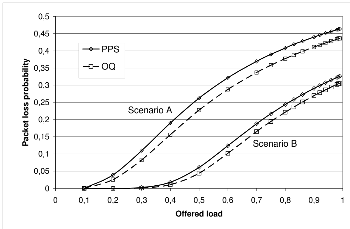
Figure 7 – Packet loss probability versus offered load in switches with finite buffer
