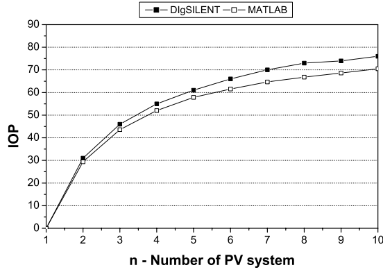
Fig. 6. Simulation results of a rural line
