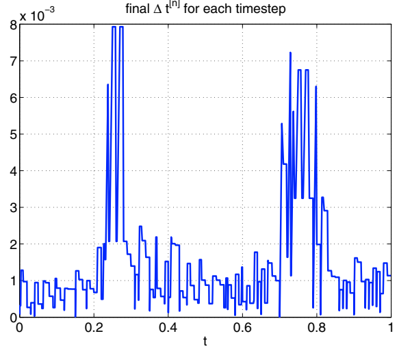
FIGURE 27. Test Problem 2: timestep-length for each timestep, \text{TOL}_\Omega = 0.2 , \text{TOL}_{I[n]} = 0.2 .
