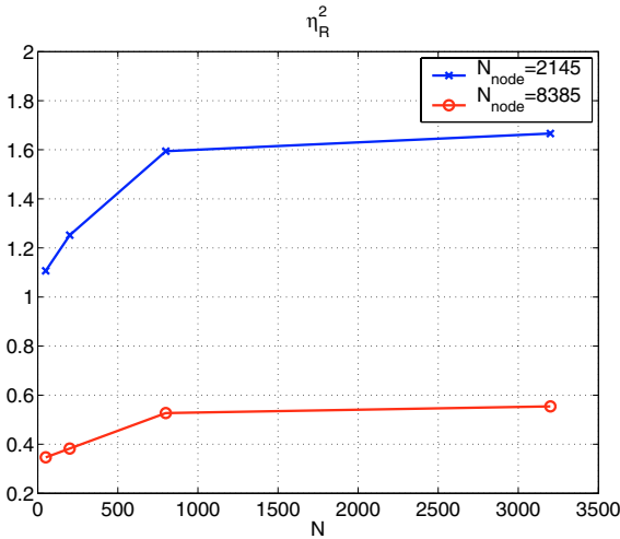
FIGURE 21. Test Problem 2: \eta_R^2 for different timesteps.
