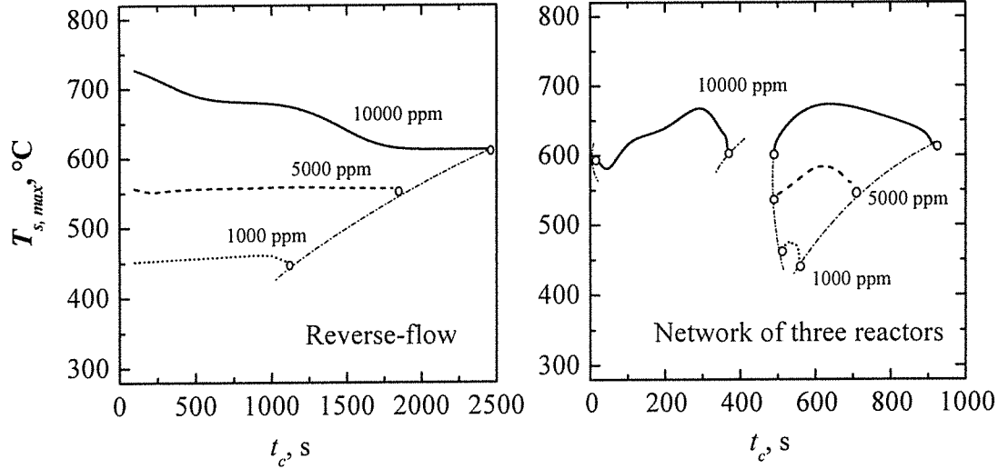
Figure 7. Comparison between the maximum temperature of the solid both for the reverse-flow reactor and for the network of three reactors for different inlet concentrations and switching times. v_R = 0.1 \text{ m s}^{-1} , L = 0.3 \text{ m} , \rho_s = 1000 \text{ kg m}^{-3} , c_{p,s} = 1000 \text{ J kg}^{-1} \text{ K}^{-1} .
